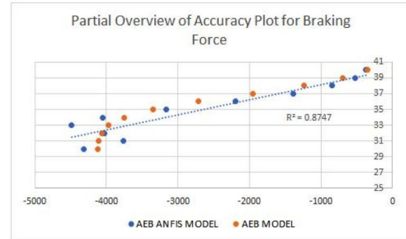
Figure 11: ANFIS result is verified with the AEB model result
