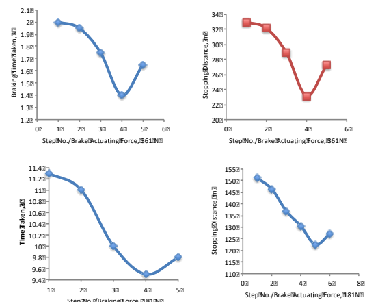
Figure 13: ANFIS controlled laboratory scale AuBS
