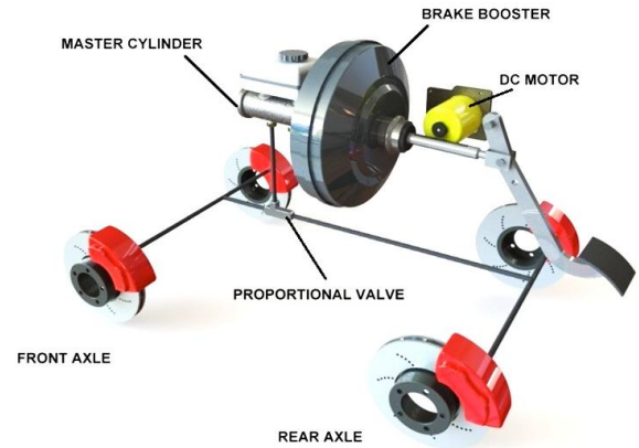
Figure 2: Architecture of Autonomous braking system
