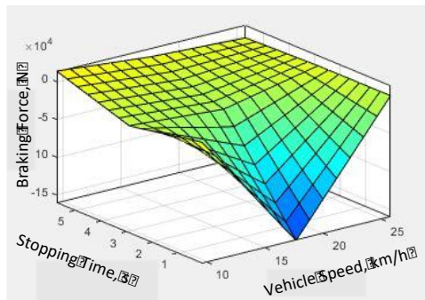
Figure 9: ANFIS simulation result for pedestrian
