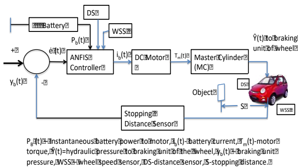
Figure 3: Basic block diagram of a closed-loop vehicle braking system
