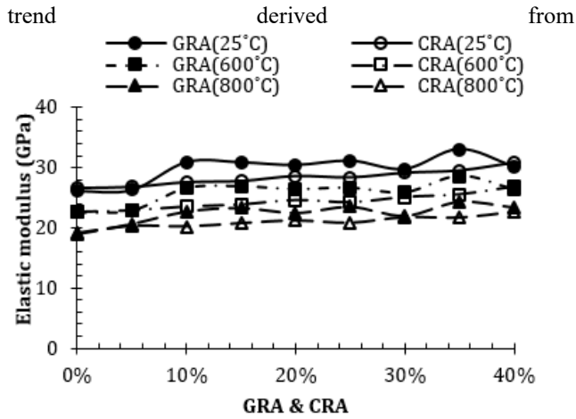
Figure 8, it is visible that with the increase in recycled ceramic and glass fines in concrete mixes, the modulus of elasticity increases in comparison with normal concrete.
