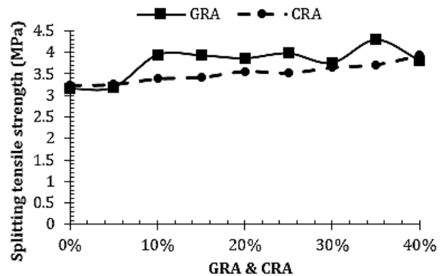
Figure 7: Splitting tensile strength of GRA and CRA concrete
