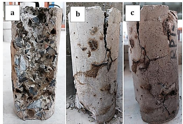
Figure 3: Concrete failures at 800°C (a) NC, (b) GRA (35%), and (c) CRA (35%)
