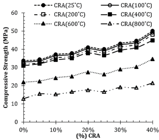
Figure 5: Compressive strength at different temperatures (CRA)
