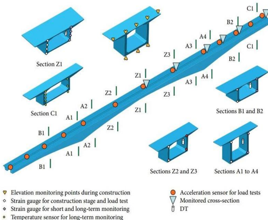
Figure 8: Sensor layout of Jing hang Canal Bridge [21]
