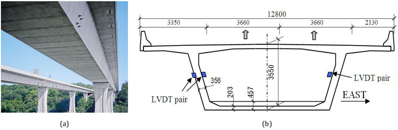
Figure 9: (a) Kishwaukee Bridge, (b) Location of LVDT sensors (unit: mm) [27]
