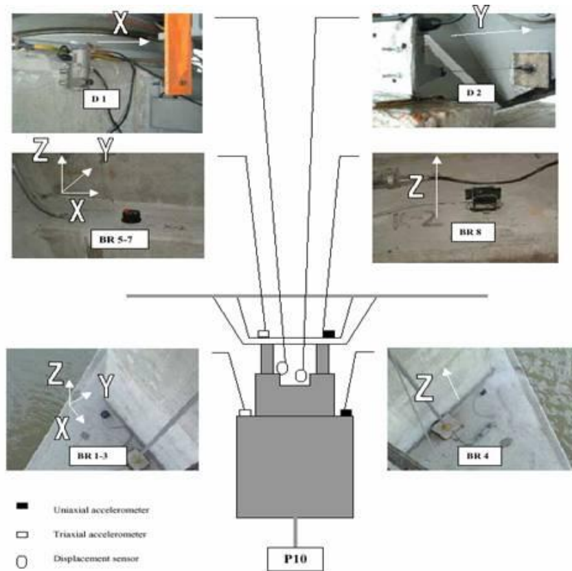
Figure 12: Location of various accelerometer and displacement sensors in Bangabandhu Bridge [28]
