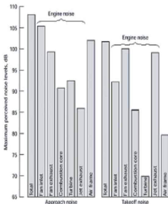
Figure 1: Aircraft relative Noise Sources [4]
