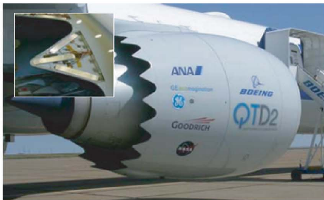
Figure 5: Variable geometry fan chevrons (inset shows individual chevron with cover removed) [15]
