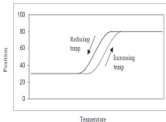
Figure 7: Position/Shape Control by SMAs (Shape Memory Alloys) [17]
