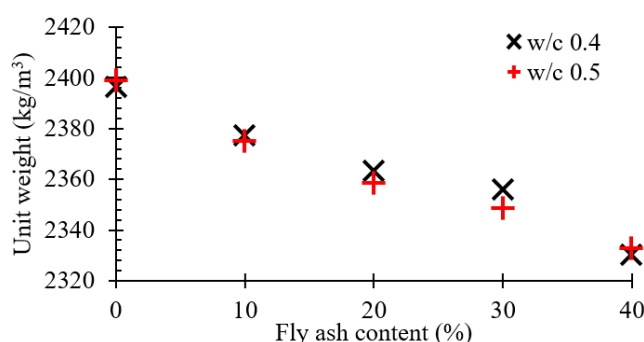
Figure 6: Unit weight for different concrete mixes
