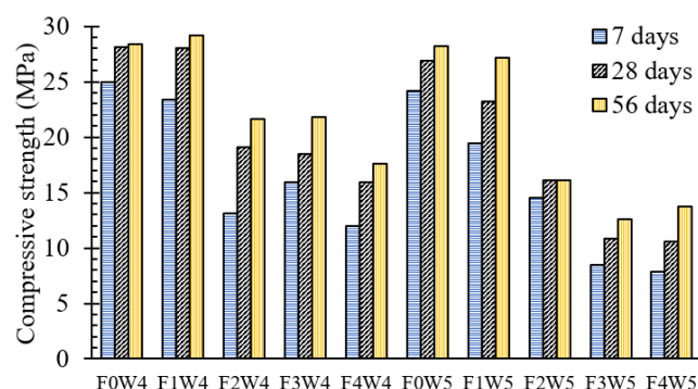
Figure 7: CS of concrete for different percentages of FA replacement
