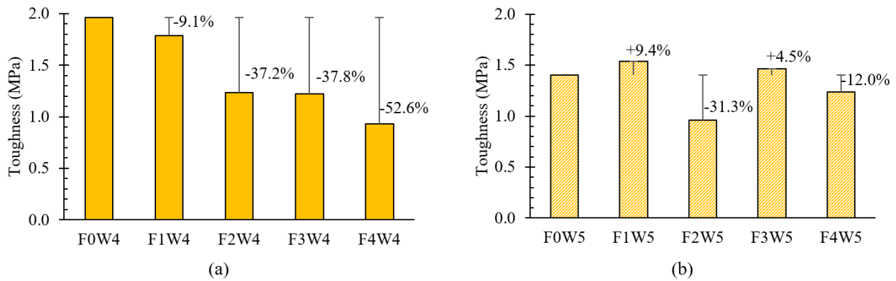
Figure 17: Toughness comparison (a) w/c ratio 0.4 (b) w/c ratio 0.5
