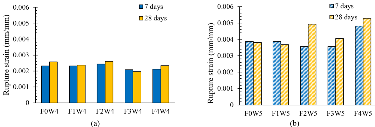
Figure 10: Rupture strain for (a) w/c ratio 0.4 (b) w/c ratio 0.5
