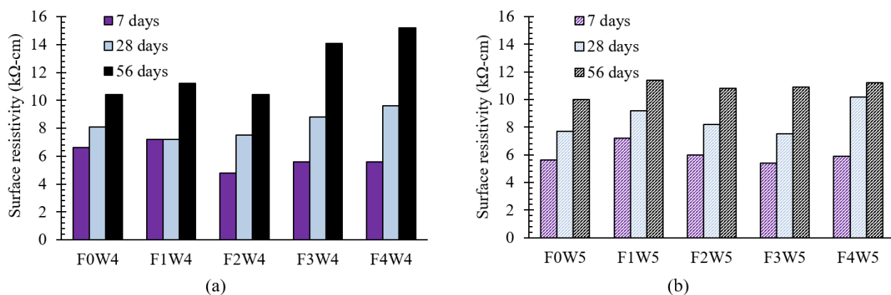
Figure 13: Surface resistivity for (a) w/c ratio 0.4 (b) w/c ratio 0.5
