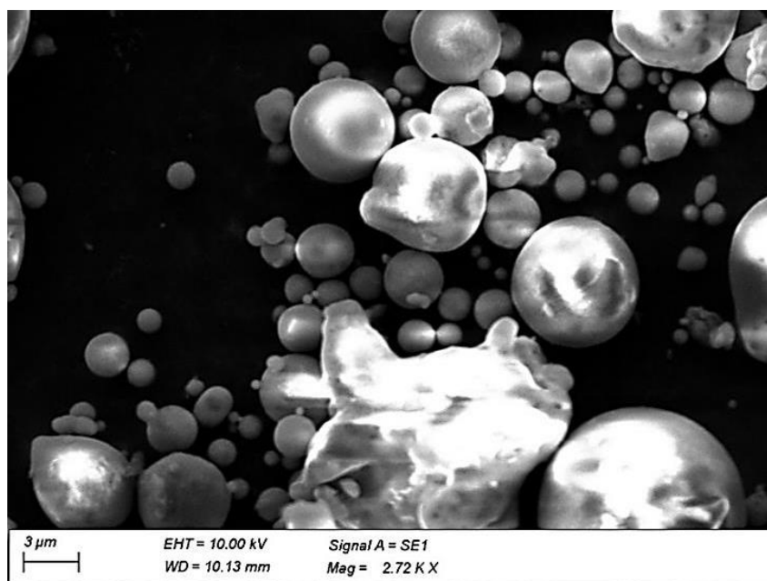
Figure 2: SEM image of FA
