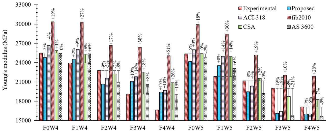
Figure 19: Percentage variation of proposed YM equation with codes prediction
