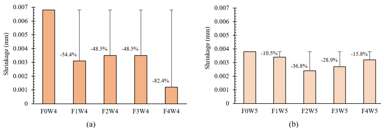
Figure 14: Shrinkage for (a) w/c ratio 0.4; (b) w/c ratio 0.5
