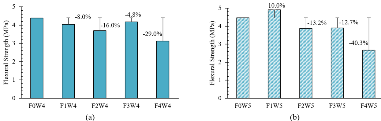
Figure 15: Flexural strength for (a) w/c ratio 0.4 (b) w/c ratio 0.5
