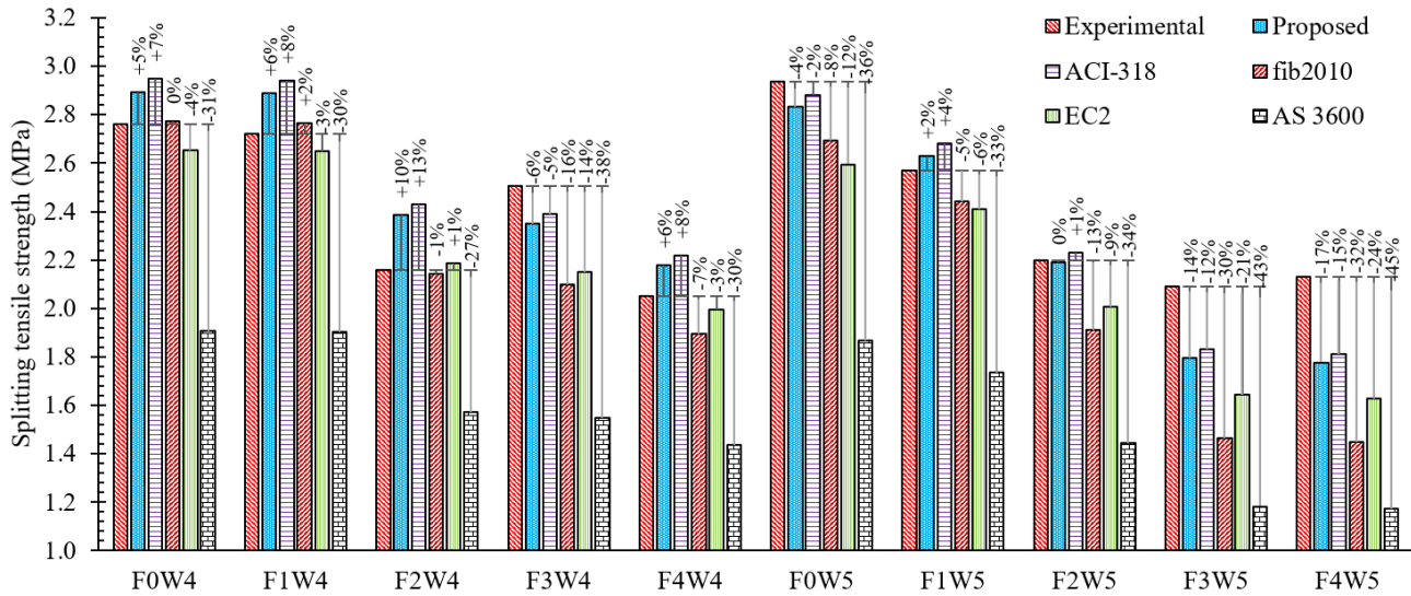
Figure 18: Percentage variation of proposed STS equation with codes prediction
