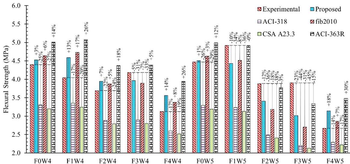
Figure 20: Percentage variation of proposed FS equation with codes prediction
