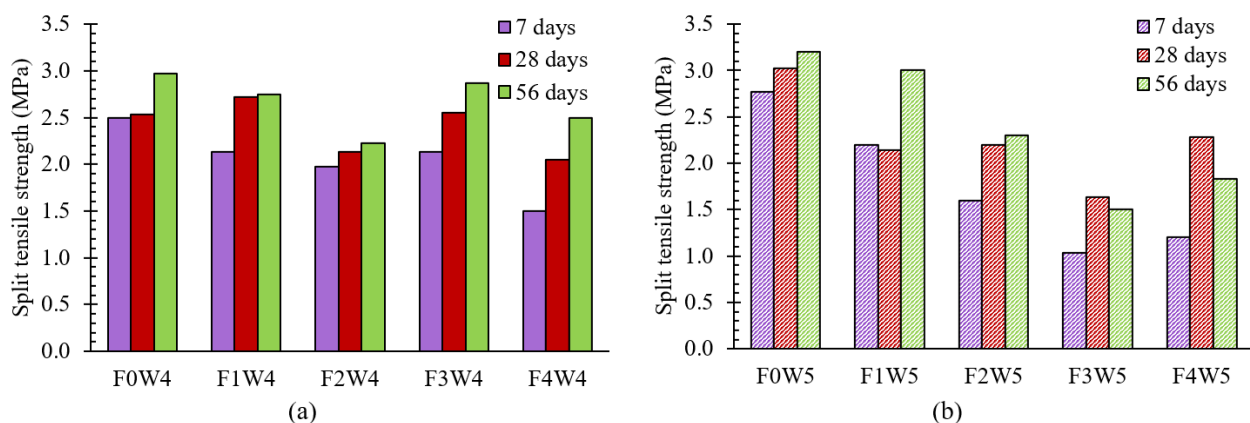
Figure 12: STS of concrete over the age (a) w/c ratio 0.4 (b) w/c ratio 0.5
