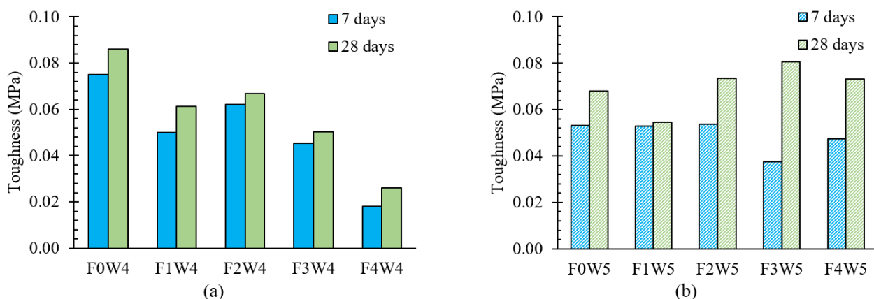
Figure 11: Toughness for (a) w/c ratio 0.4 (b) w/c ratio 0.5
