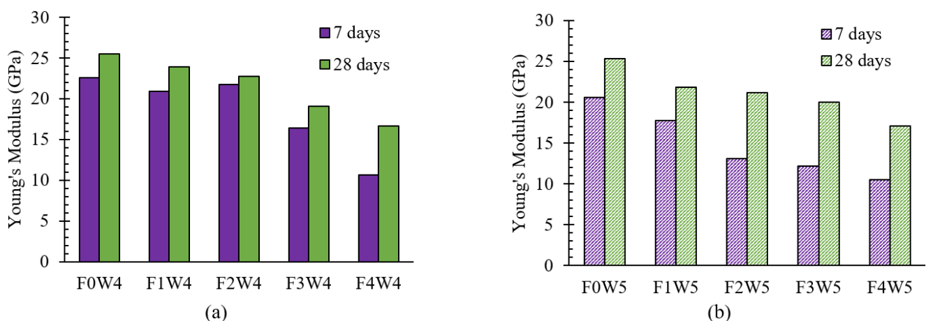
Figure 9: Young's modulus for (a) w/c ratio 0.4 (b) w/c ratio 0.5
