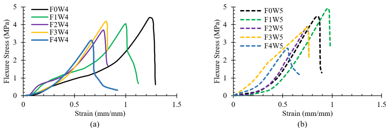
Figure 16: Stress vs. strain plot for (a) w/c ratio 0.4 (b) w/c ratio 0.5
