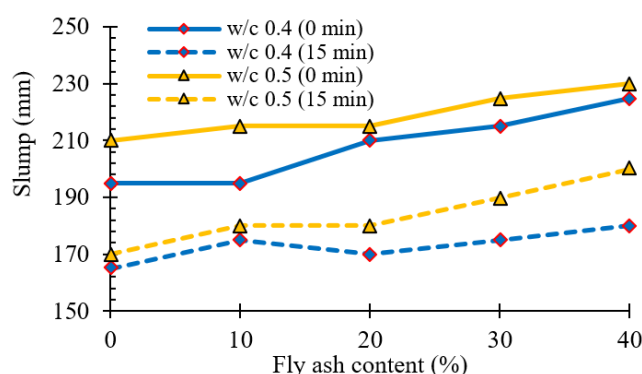
Figure 5: Slump height for different mixes
